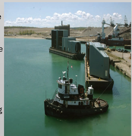
Parts of units 3 & 4 ductwork for the Monroe Power Plant.
